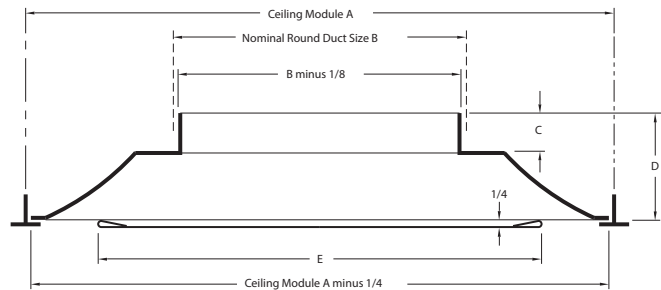
Frame Type 3 Full Face (Lay-In)
